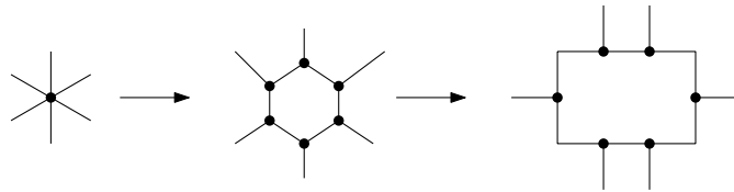
ABBILDUNG 1: Replacement of a vertex of higher degree by a ring, which shall be represented by a rectangle in the orthogonal drawing.
